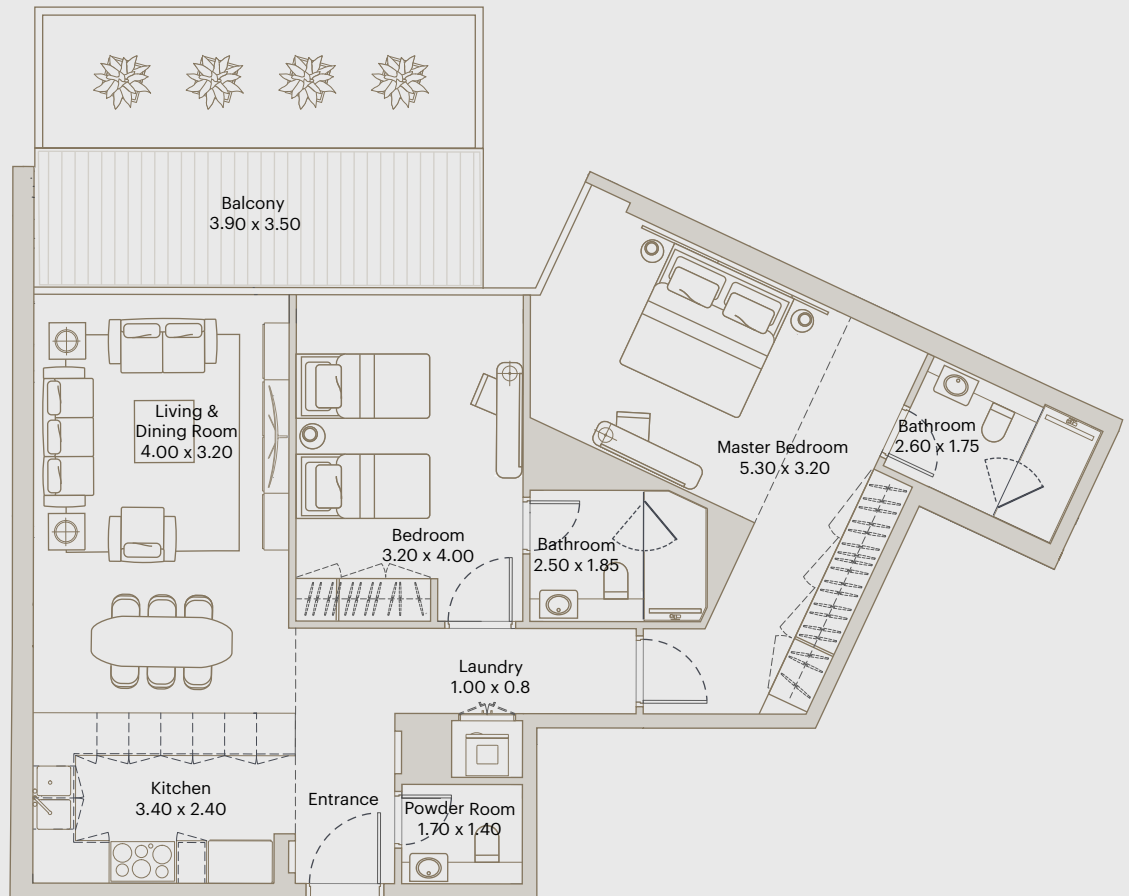
FLAT 17 @ 3RD, 5TH, 7TH, 9TH, 11TH, 13TH, 15TH & 17TH FLOOR
