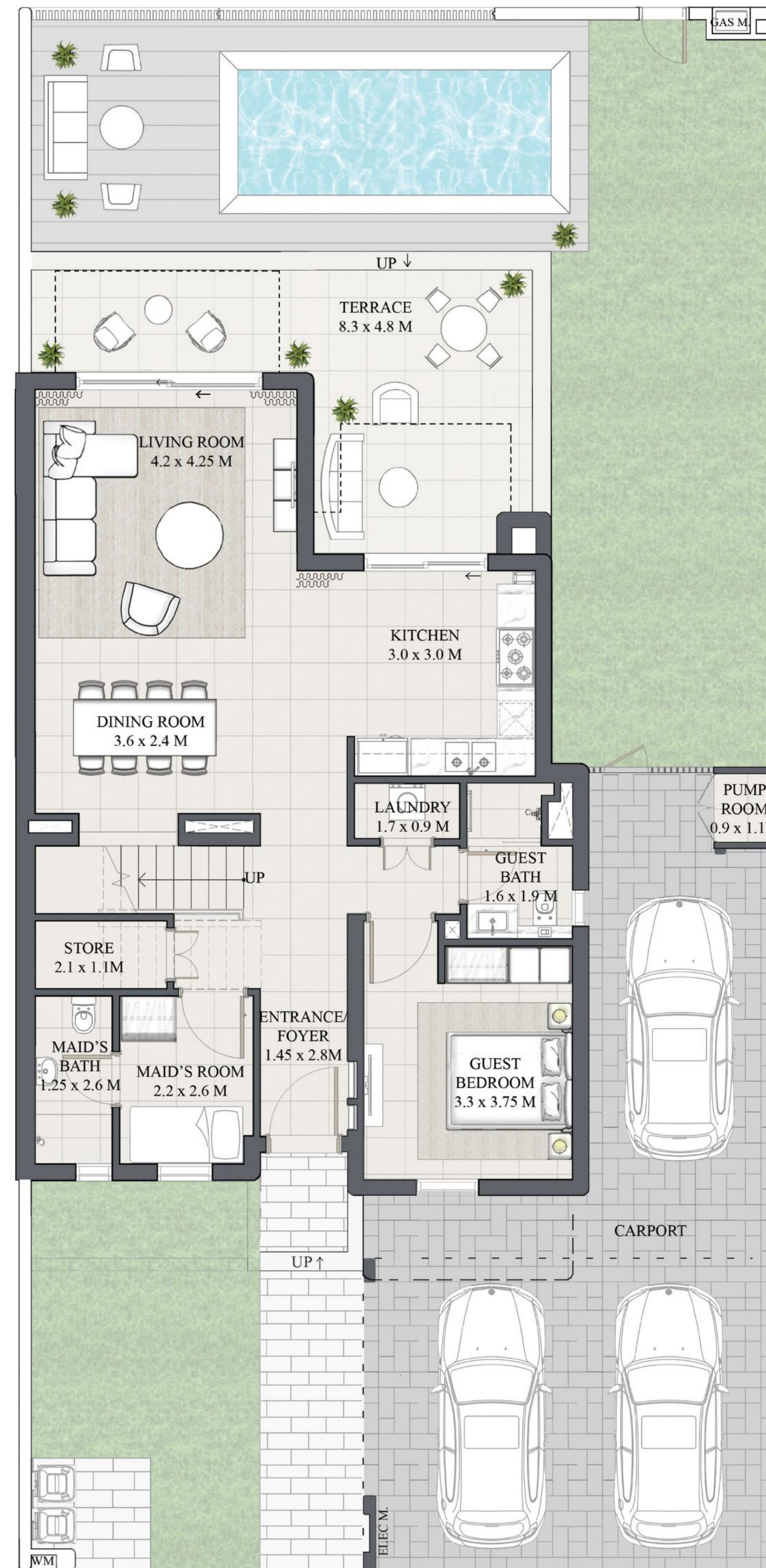
GROUND FLOOR
