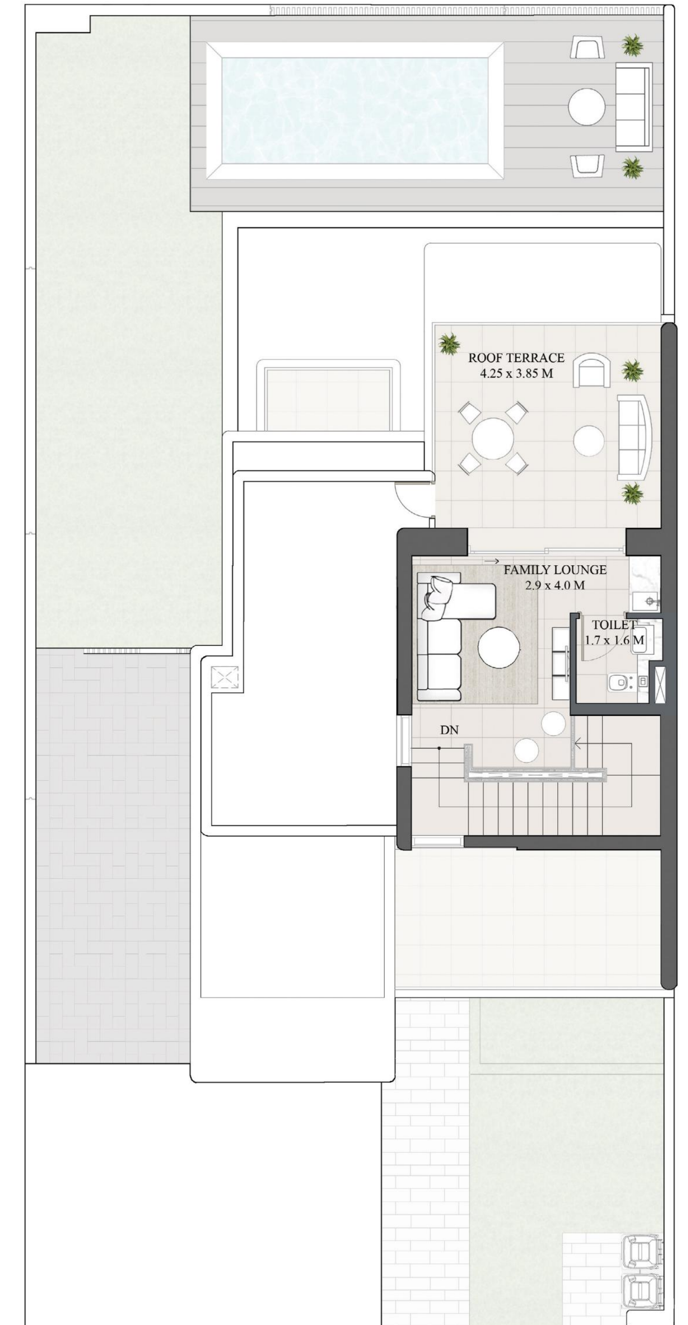
ROOF FLOOR
